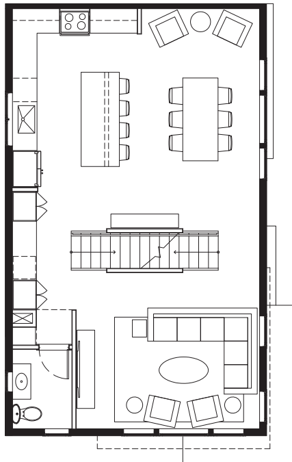
LIVING LEVEL
